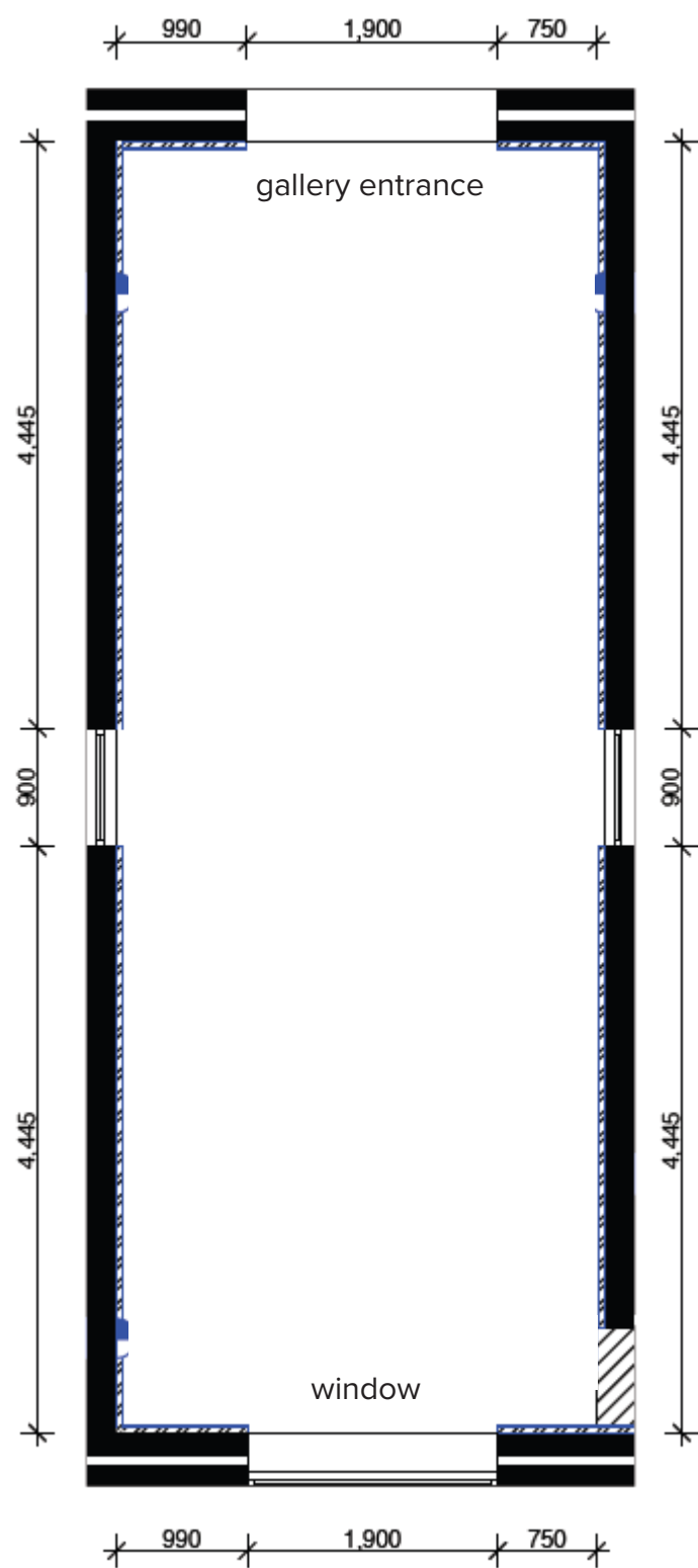
floor plan
