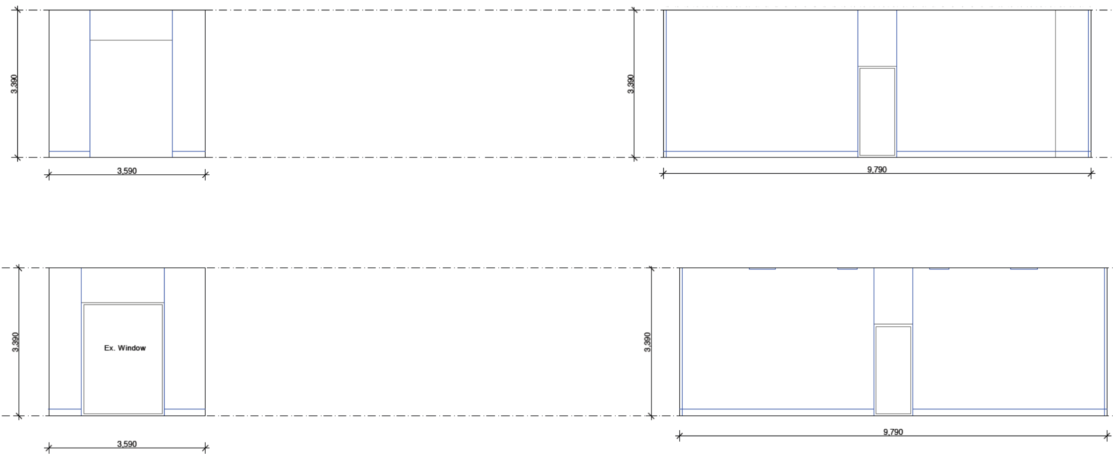
elevations
